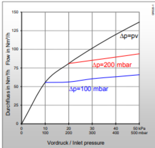
Example flow rate type: GRS25-VA G1 F/F. Values for other connections on request.
